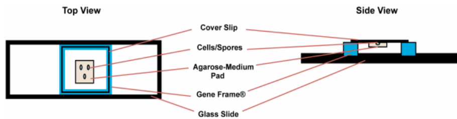
Figure 1. Closed air-containing chamber for live cell imaging
