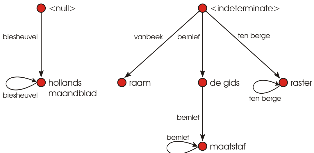
Figure 1 - Example of a transition network.
