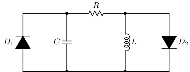
Fig. 6. RLC circuit with ideal diodes
